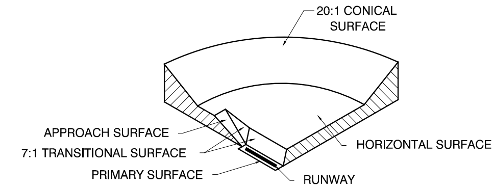
TYPICAL FAR PART 77 SURFACES
