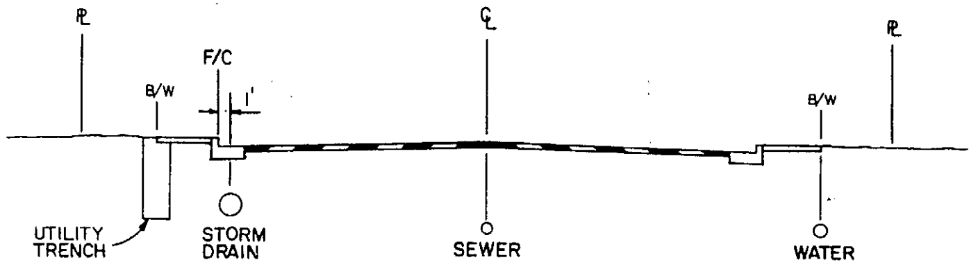
TYPICAL UNDERGROUND INSTALLATION FOR COMMERCIAL, INDUSTRIAL & URBAN DEVELOPEMENTS
