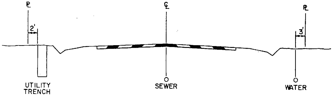
TYPICAL UNDERGROUND INSTALLATION FOR ESTATE, RURAL & AGRICULTURAL DEVELOPEMENTS
